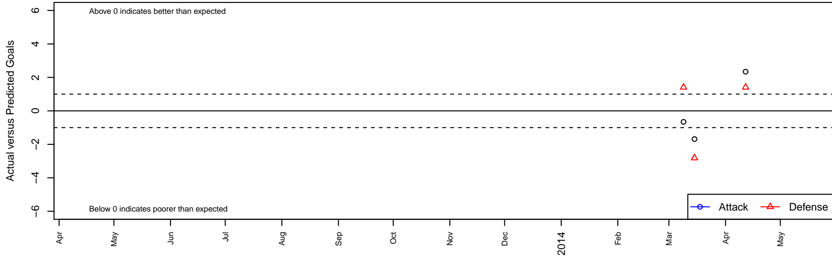
Gorge FC B99 Dots are actual minus expected GF (blue circles) and GA (red triangles). Blue line is smoothed change in attack strength. Red is smoothed change in defense strength.
